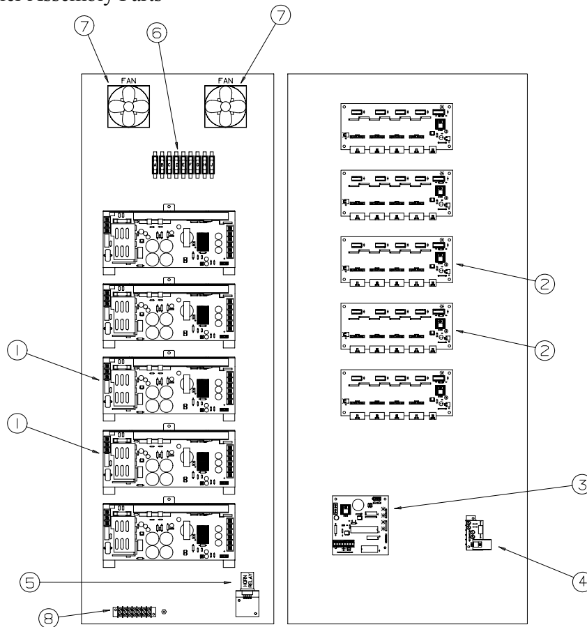
figure 2 CONTROLLER ASSEMBLY
