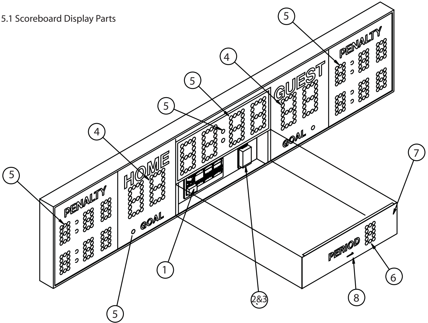
Figure 1 DISPLAY ASSEMBLY
