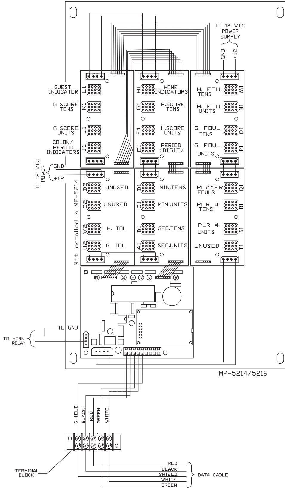
CONTROLLER WIRING
