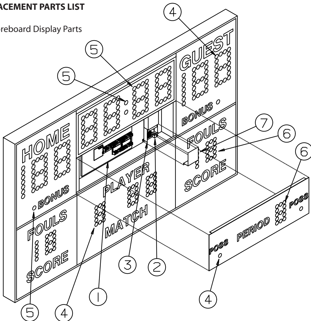
Figure 1 DISPLAY ASSEMBLY
