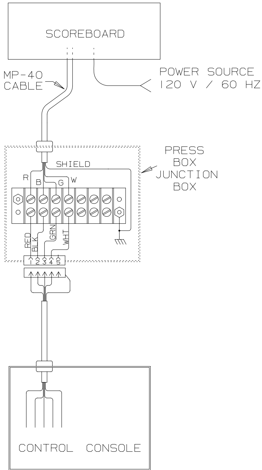
SYSTEM LAYOUT
