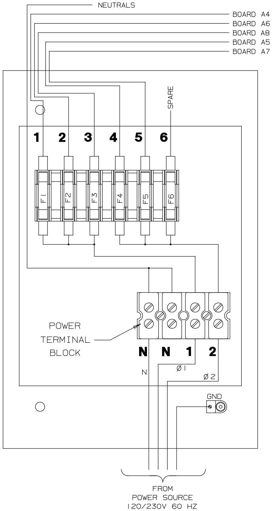
POWER WIRING
