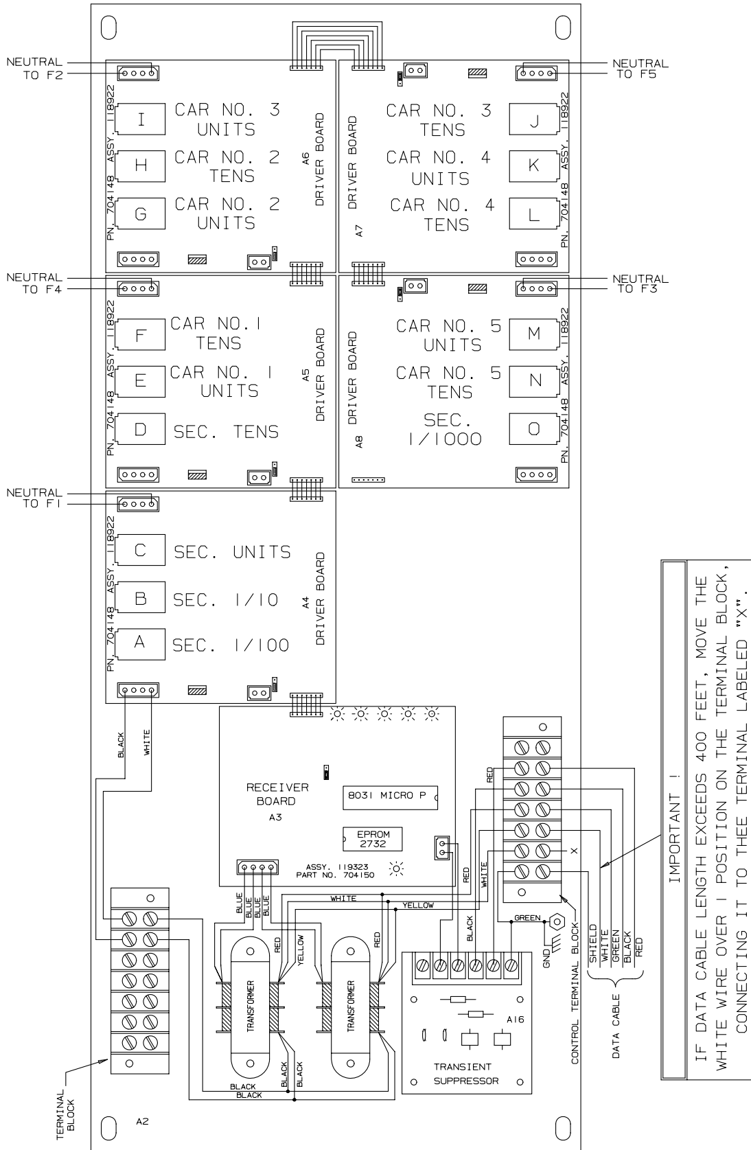
CONTROLLER ASSEMBLY
