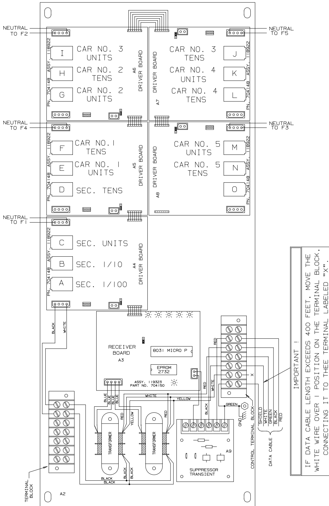
CONTROLLER ASSEMBLY
