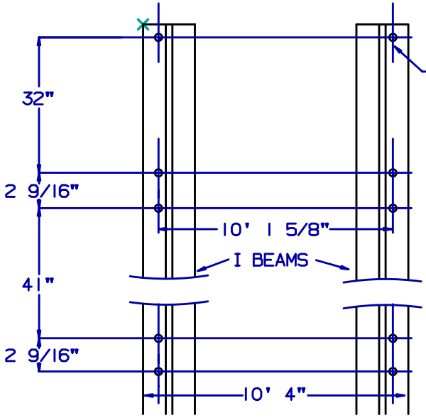
FRONT VIEW MOUNTING DETAIL
