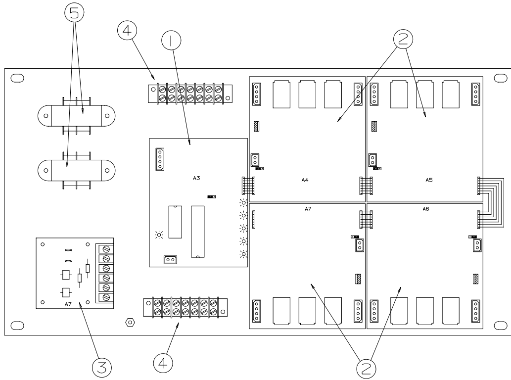
figure 2 CONTROLLER ASSEMBLY
