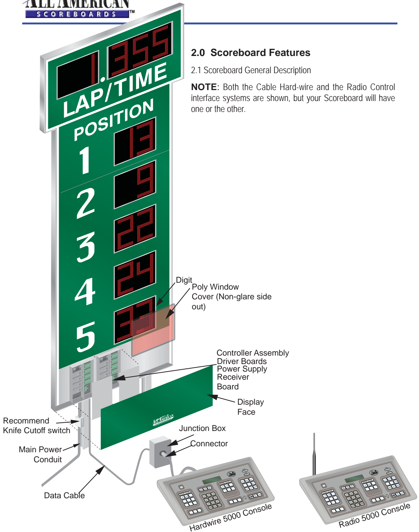
Figure 1: General Assembly of Scoreboard System
