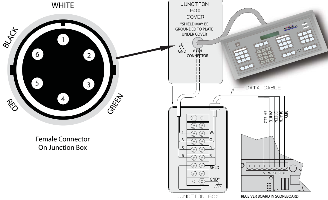
Single Scoreboard Wiring
