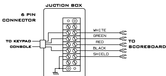
Figure 3: Junction Box (Cable Hard-wire System only)
