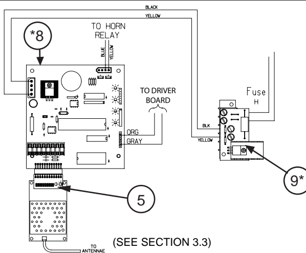
Figure 4: Version 2 Controller Board (SEE SECTION 3.3)
