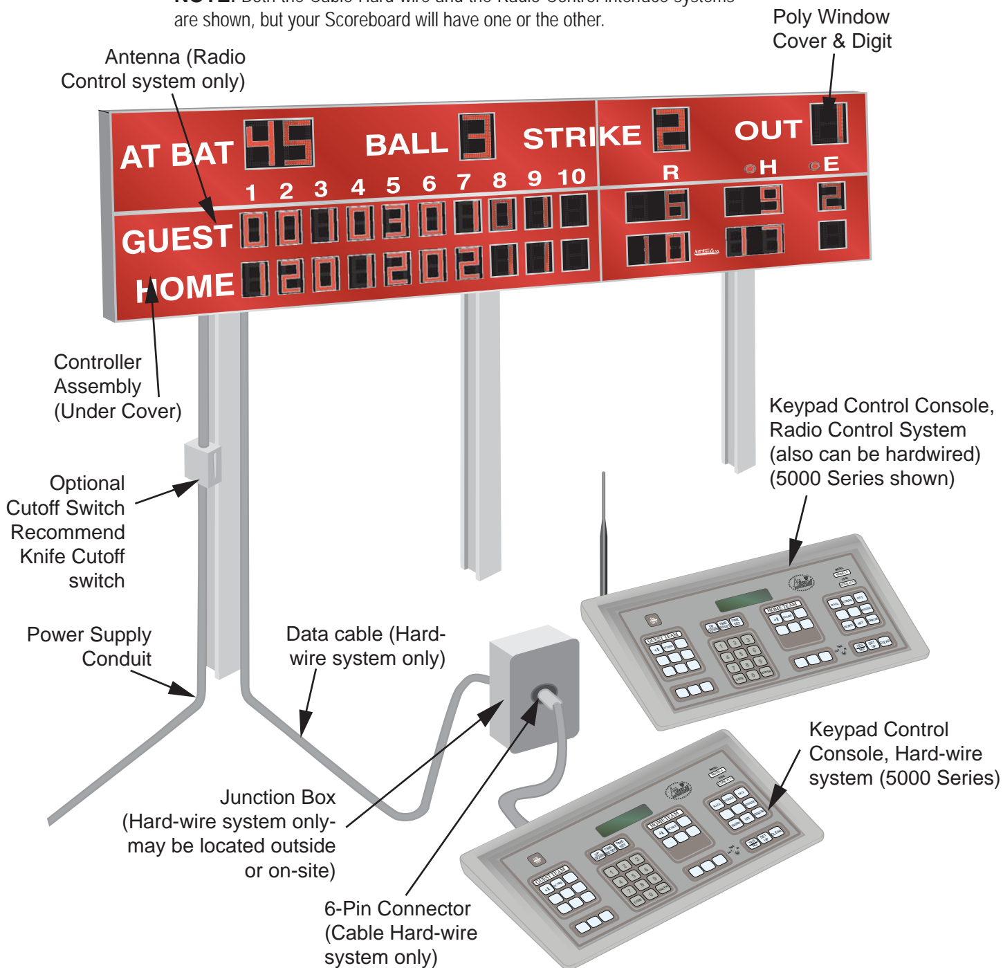
Figure 1: General Assembly of Scoreboard System (MP-7479 Shown)
