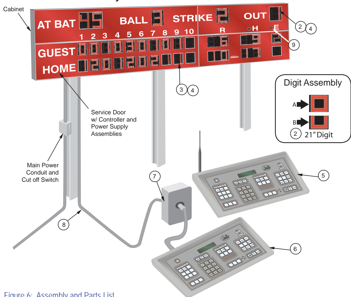
Figure 6: Assembly and Parts List
